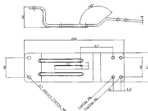
01 sb60-staffa portabracciolo sb60-support of arm
