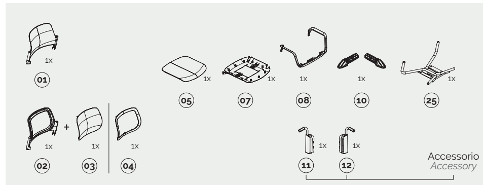
swivel frame - with armrests
