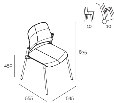
4-legs frame - without armrests
