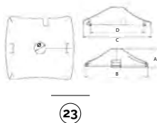
CPG plastic cover for swivel frame
