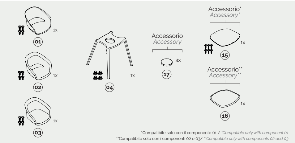
kit 4 gambe in plastica / plastic 4-leg kit
