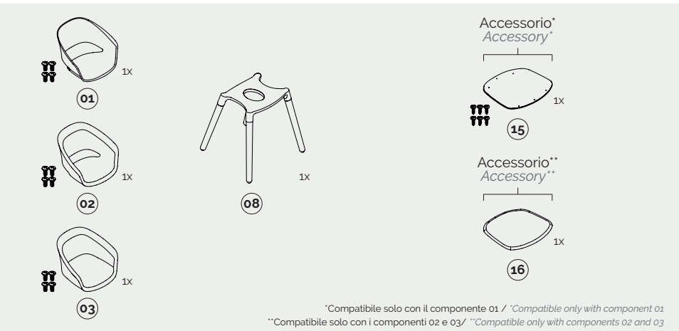
kit 4 gambe in legno / wooden 4-leg kit
