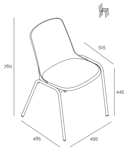
versione 4 gambe Conference 4-leg Conference version
