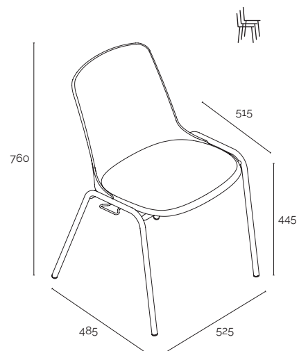
versione 4 gambe Conference con ganci 4-leg Conference version with hooks
