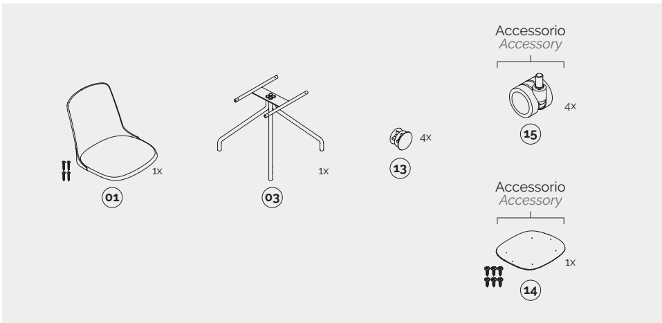
kit 4 razze / 4-spoke kit
